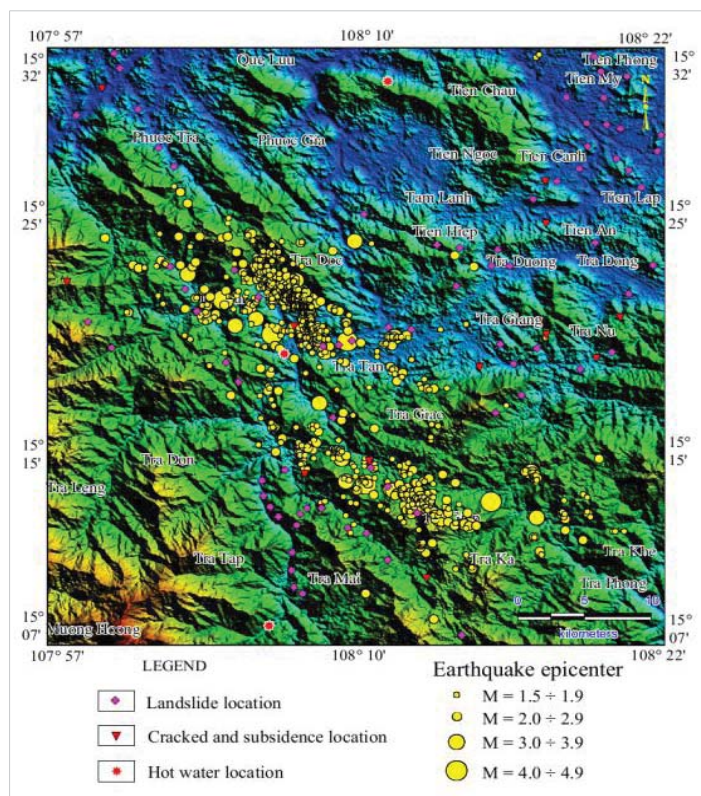
Figure 3: Distribution of earthquake epicenters in the ST2 region3z.
