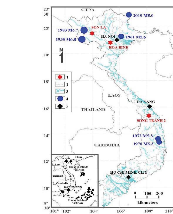
Figure 1: Location of Son La, Hoa Binh and Song Tranh 2 hydropower reservoirs on the map of Vietnam. (1-study areas; 2-border lines; 3-rivers; 4-earthquake; 5-places)"
